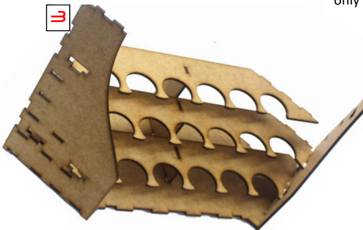
3 glue on the 2 side walls, tabs all the way in.
