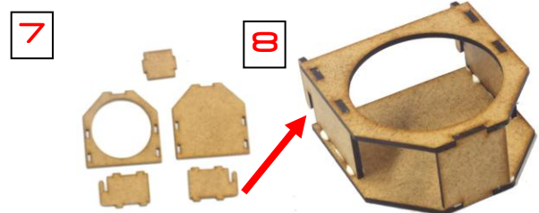
7-8 Water pot holder: Glue the 2 sides, top, bottom and front pieces together, little tabs facing to the back. Slide over front support strip.
