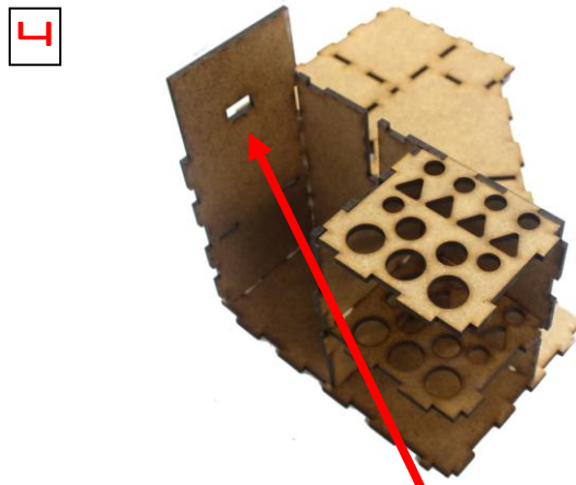
4 then glue in the tall wall (hole towards the top) and glue the whole sub-assembly into the slits of the base plate, together with the 2 little front pieces in step 5.
